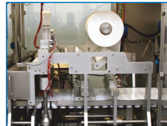
SEALING STATION
